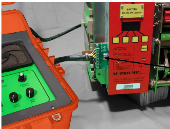
Figure 3 Test Set Connected to legacy AC-PRO-MP (side test port)
